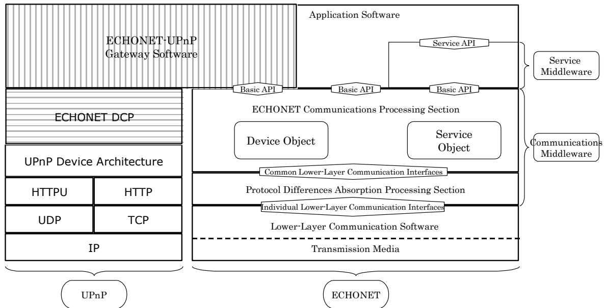
Fig. 1.1 Relationship between the ECHONET Lite-UPnP Gateway Software and Other Communication Layers
