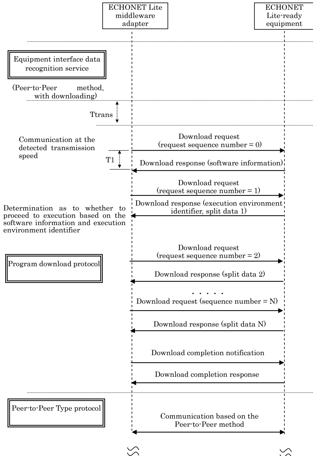
Fig. 3.30 Program Download Communication Sequence
