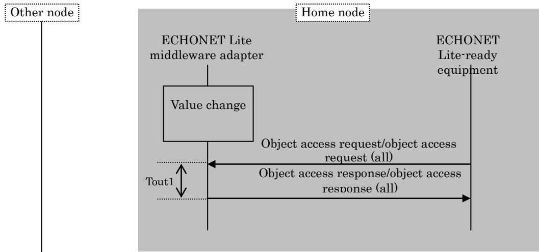
Fig. 3.26 Object Access Request Sequence
