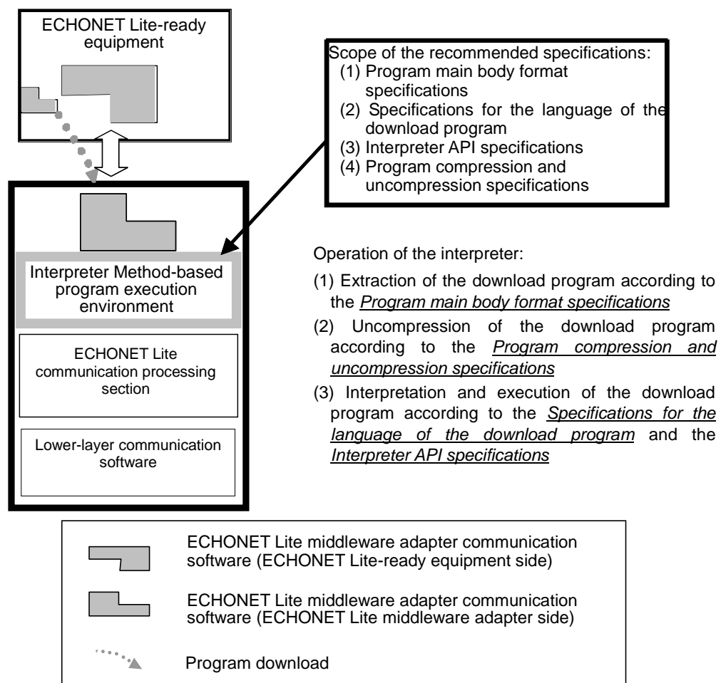
Fig. 3.31 Scope of the Recommended Specifications
