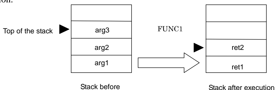
Fig. 3.38 Stacks before and after Execution of API
