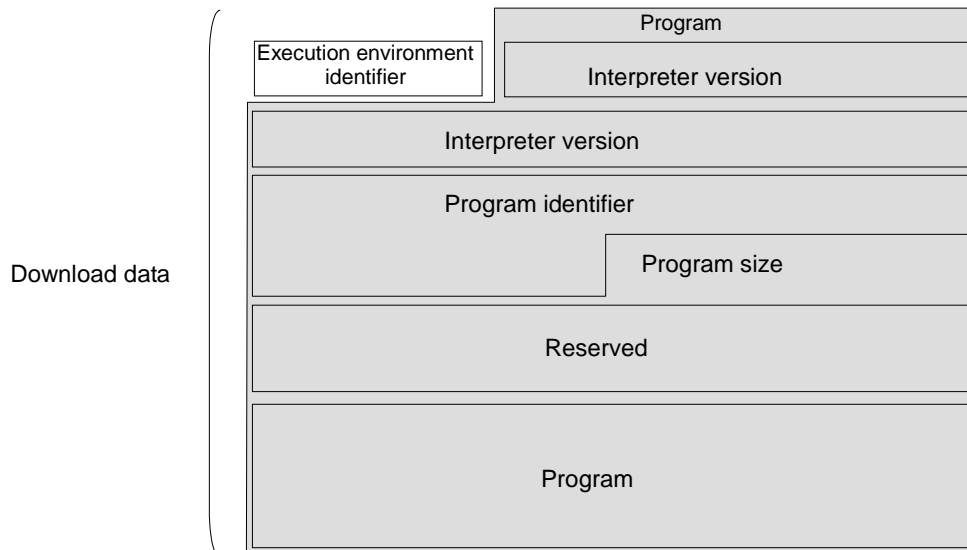
Fig. 3.35 Format of the Main Body of the Program
