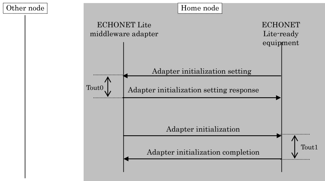
Fig. 3.21 Initialization Sequence
