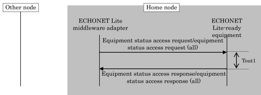
Fig. 3.24 Equipment Status Access Request Sequence
