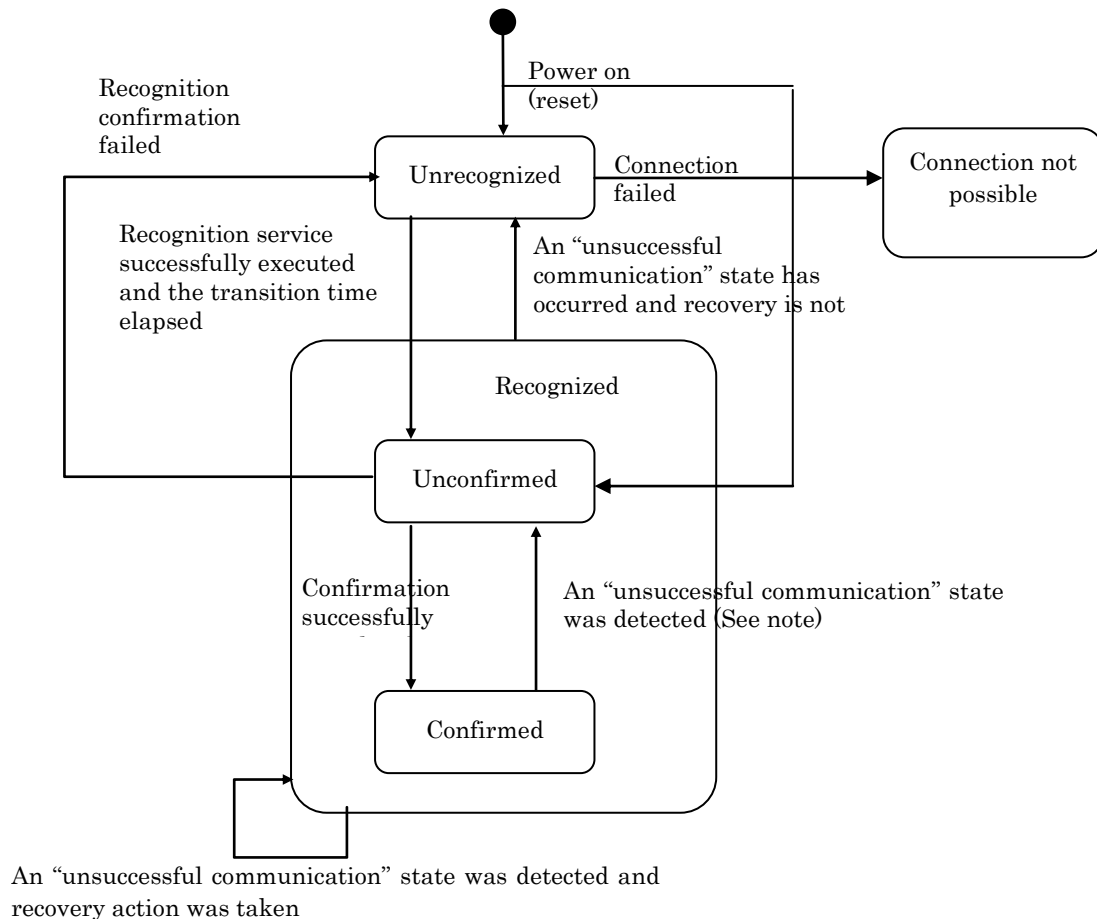
Fig. 3.13 Status Change Diagram
