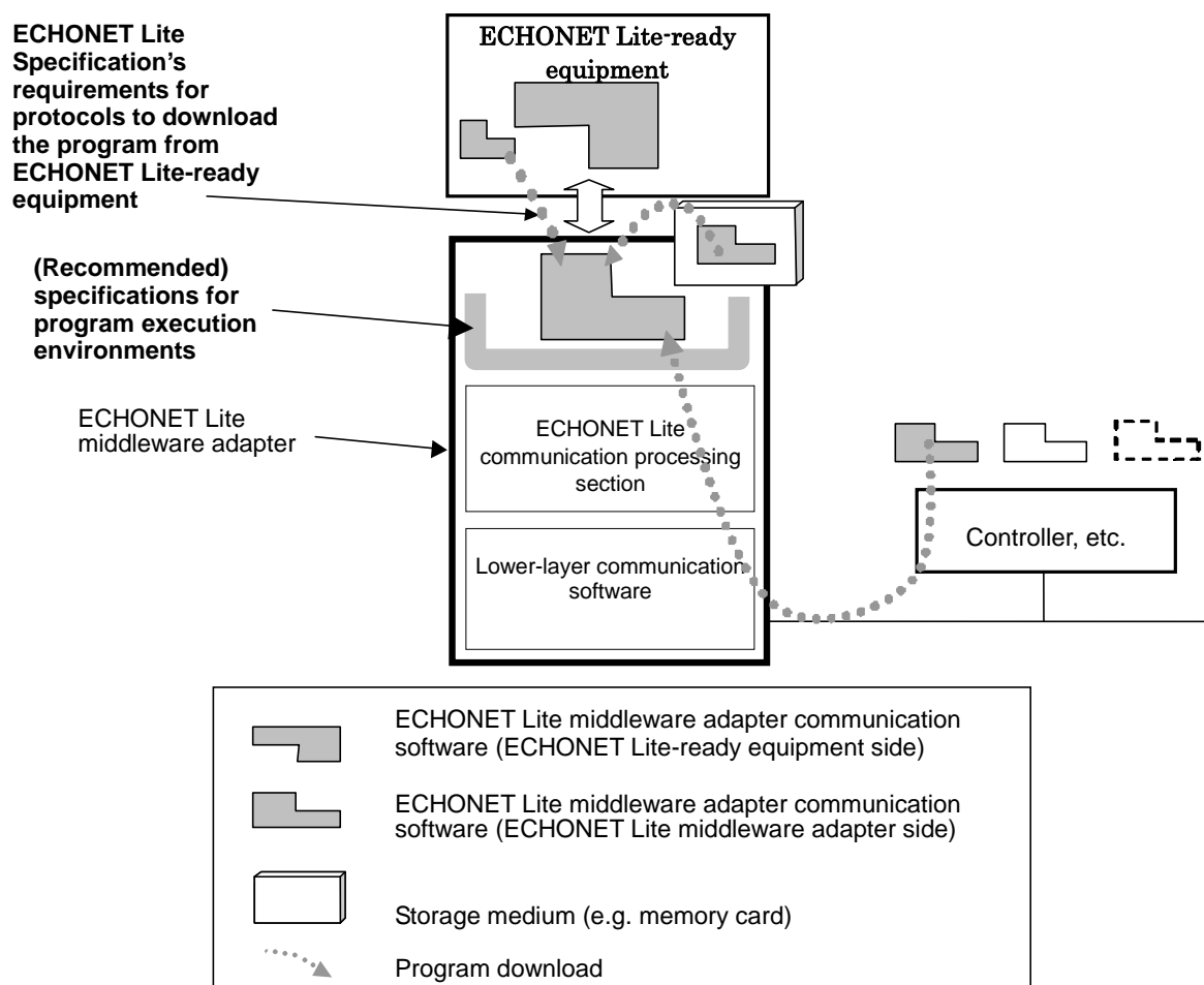
Fig. 3.27 Scope of the ECHONET Lite Specification with Regard to the Program Download Method
