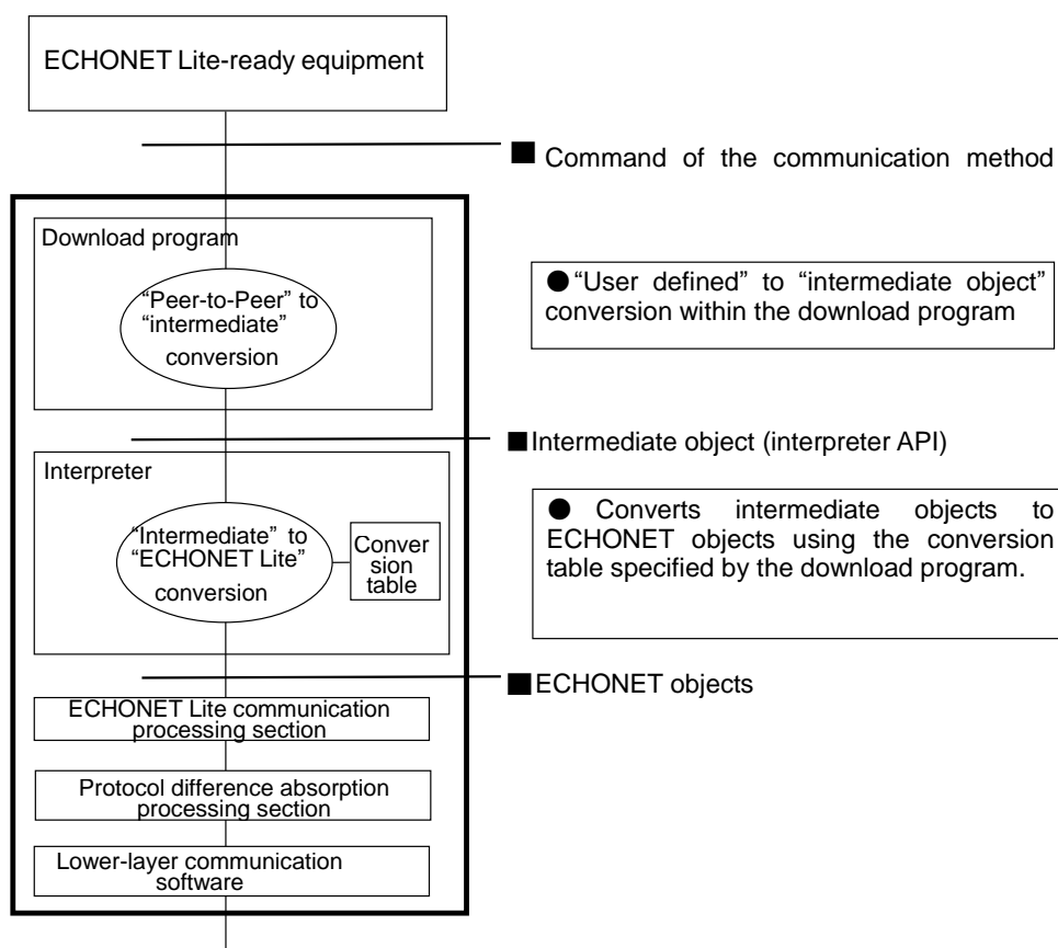
Fig. 3.32 Roles of the Download Program and the Interpreter
