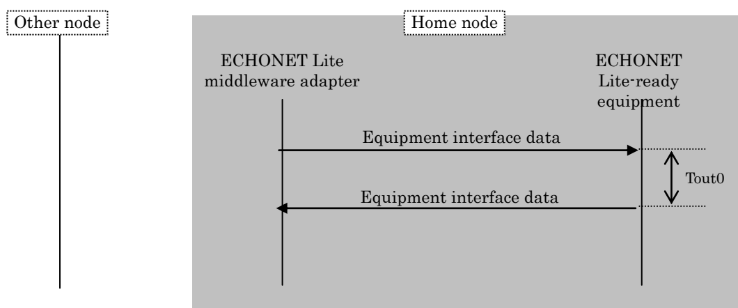
Fig. 3.20 Data Confirmation Sequence
