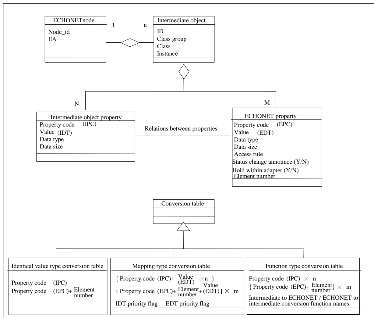
Fig. 3.34 Overview of the Conversion Table Model
