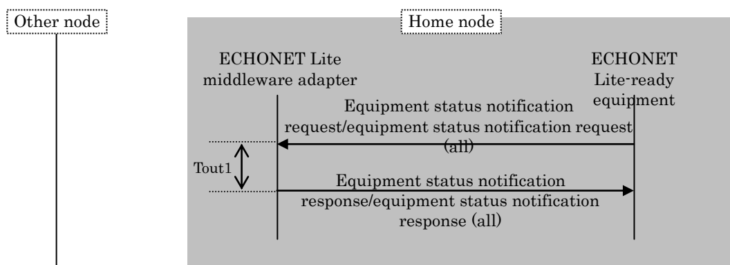
Fig. 3.25 Equipment Status Notification Request Sequence
