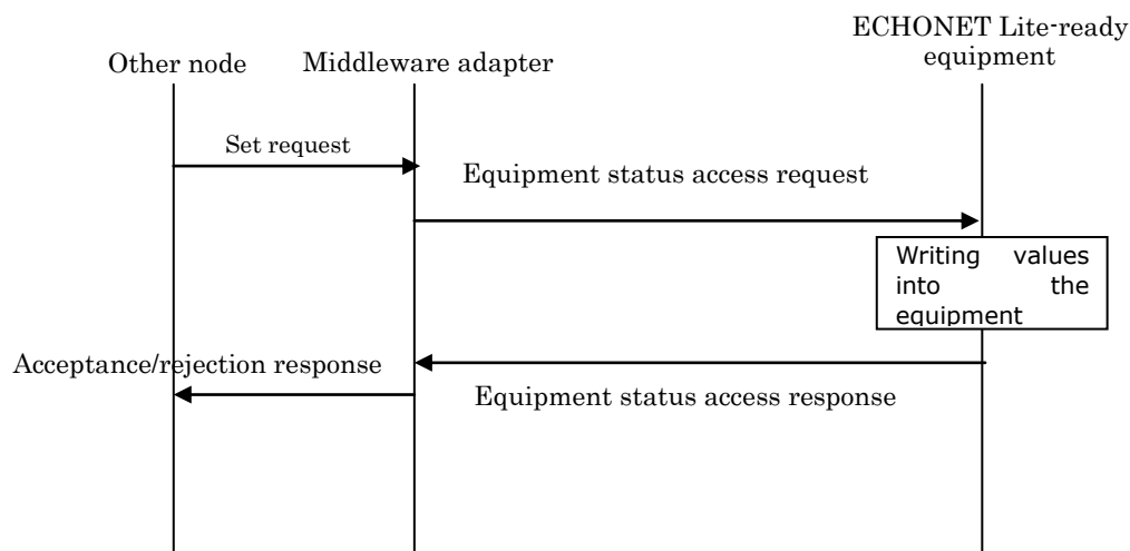
Fig. 3.16 Operation of IASetup
