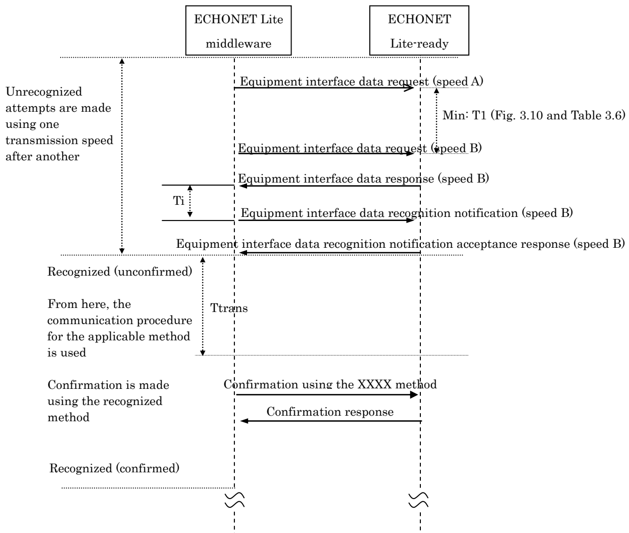
Fig. 3.12 Operation Sequence
