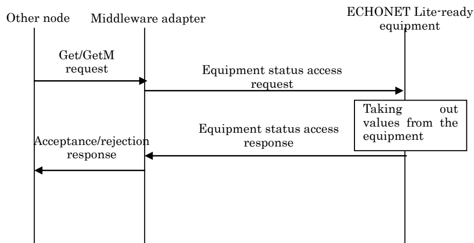
Fig. 3.18 Operation of IAGetup
