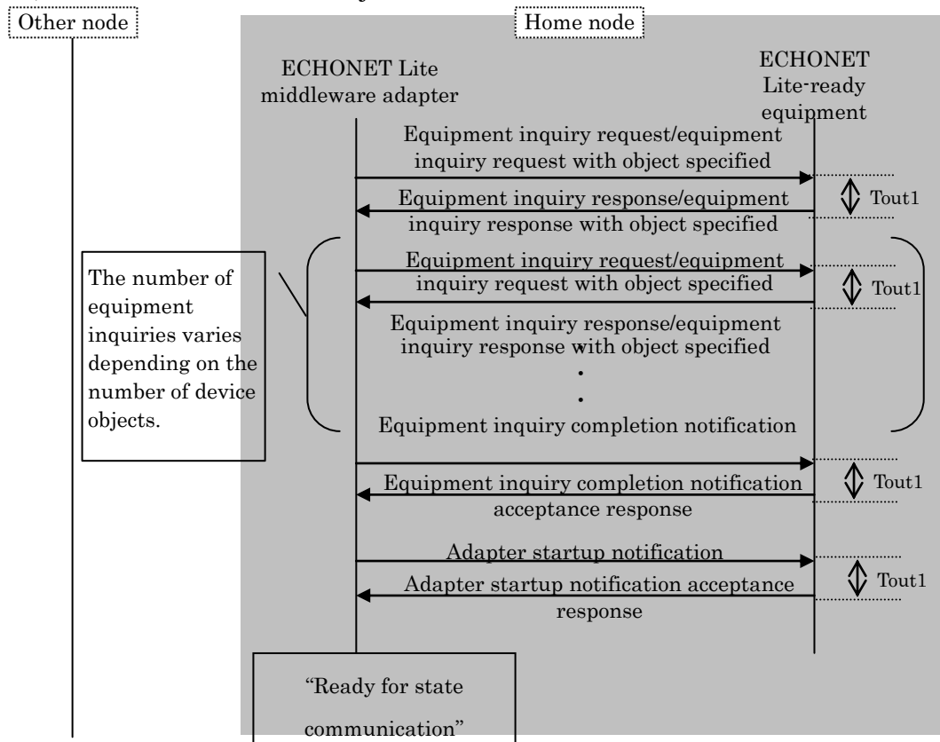
Fig. 3.23 Object Operation Sequence (2)
