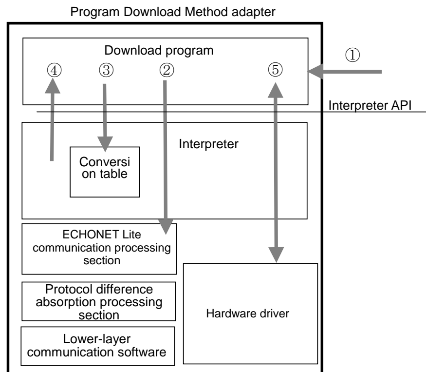
Fig. 3.33 Operation Procedure
