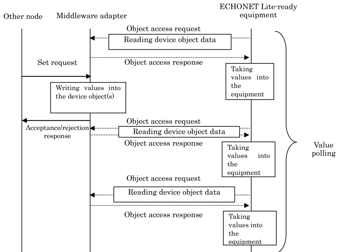
Fig. 3.15 Operation of IASet
