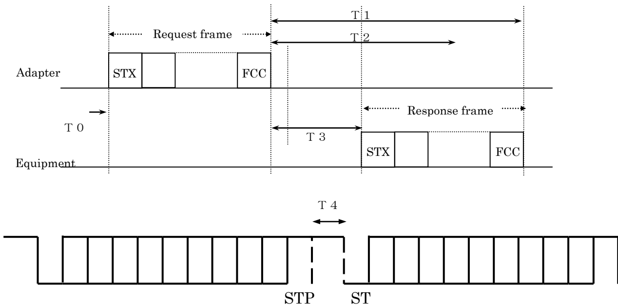
Fig. 3.10 Timing Requirements
