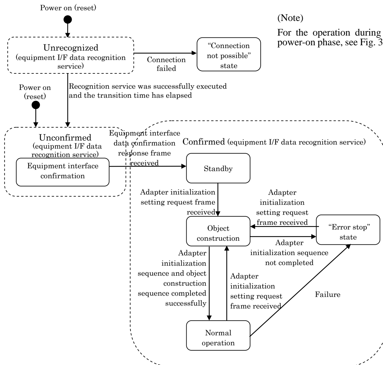
Fig. 3.19 Middleware Adapter Status Changes
