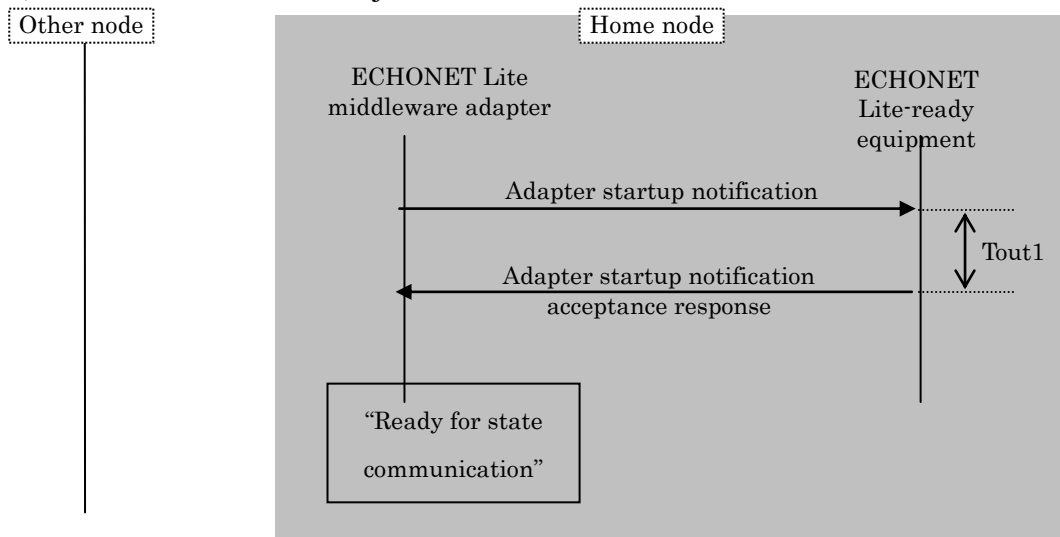
Fig. 3.22 Object Operation Sequence (1)
