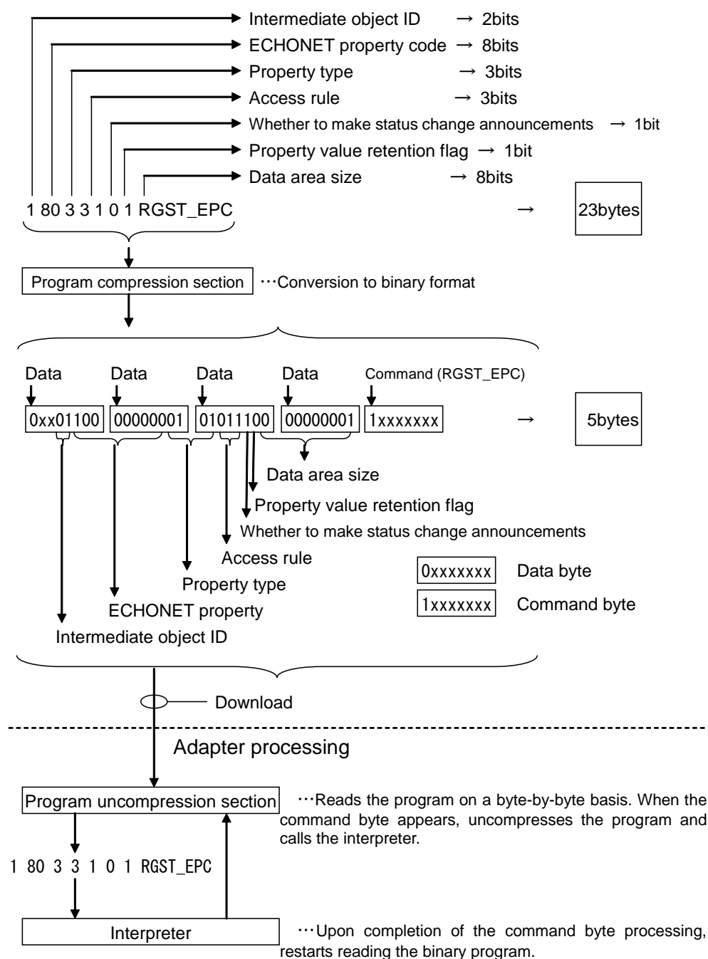
Fig. 3.42 Overview of Program Compression
